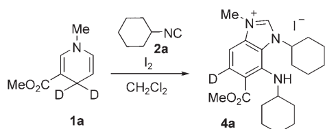
Scheme 2. Synthesis of deuterated 4a from 4,4-dideuterated DHP 1a .
